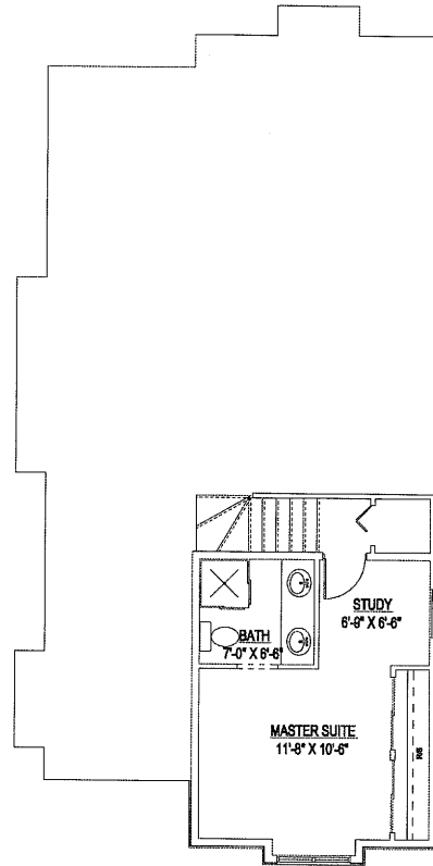
UPPER FLOOR
