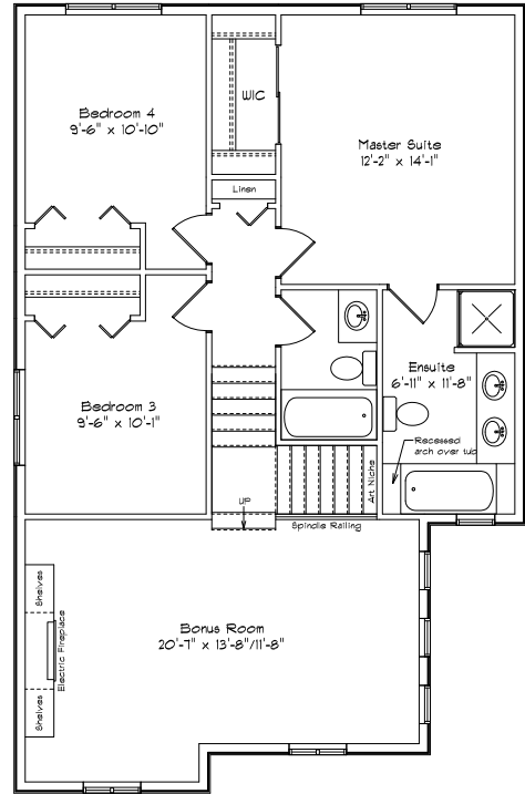
UPPER FLOOR
